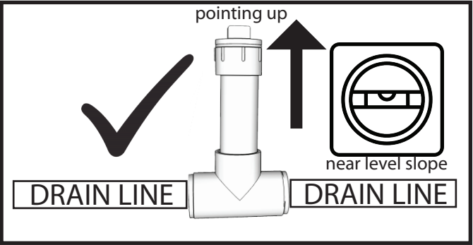
FIG. 2 Orient the Chlorinator and drain line at a near level position.
